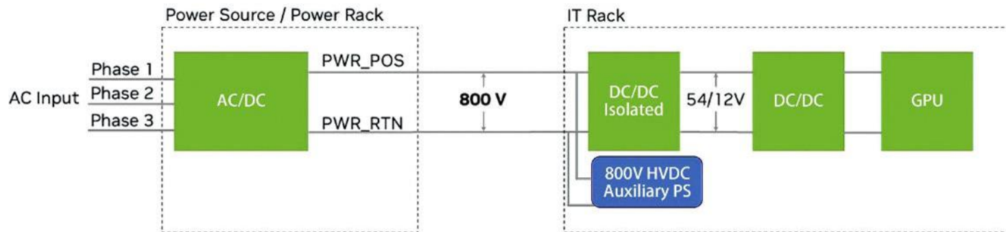
800V HVDC Auxiliary Power
